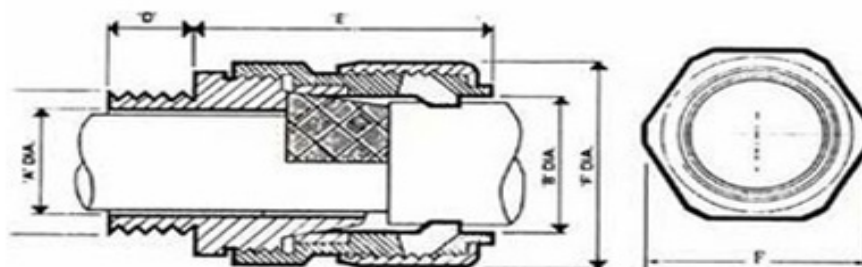
BRASS CX TYPE CABLE GLANDS
