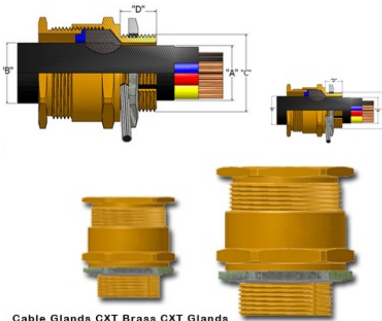
Cable Glands CXT Brass CXT Glands
