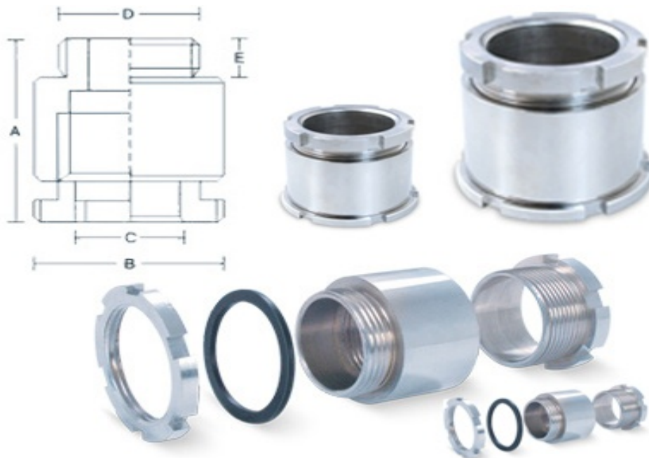
Marine Cable glands Brass Cable Glands Marine
